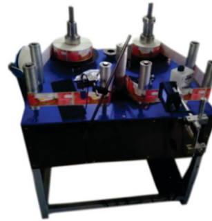
WINDER/REWINDER
